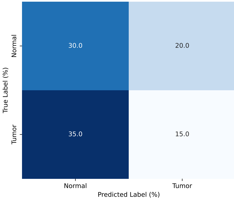
Confusion Matrix: Baseline (Underfit)
